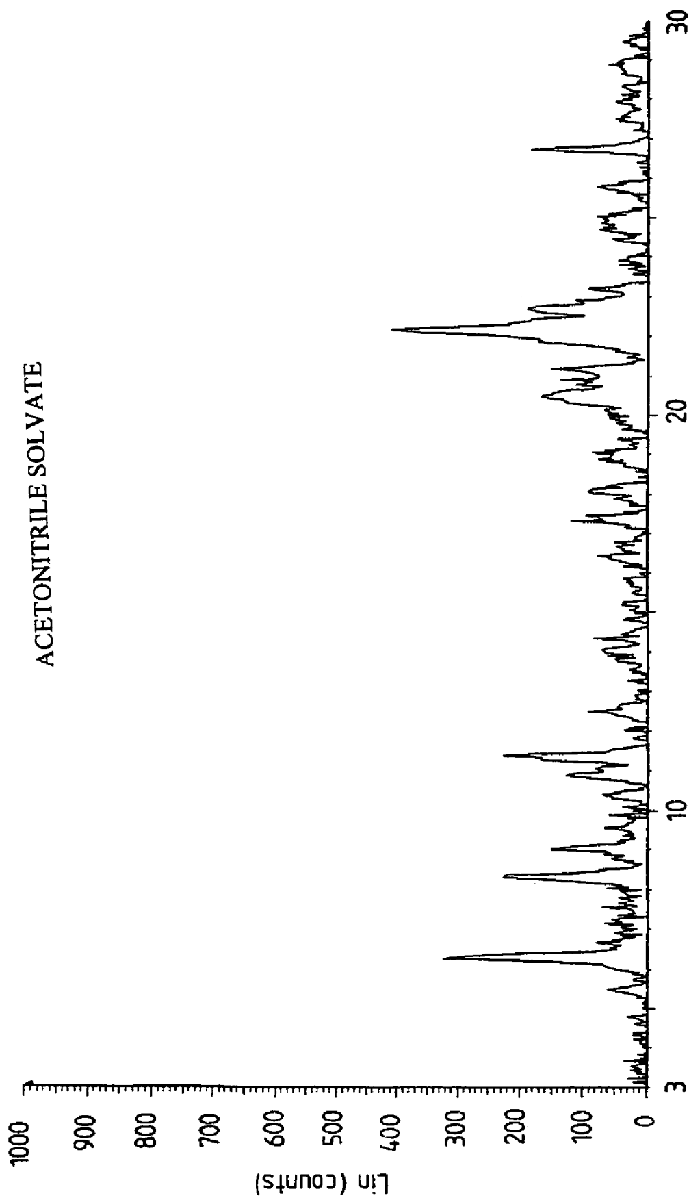
2-Theta-scale FIG.13
