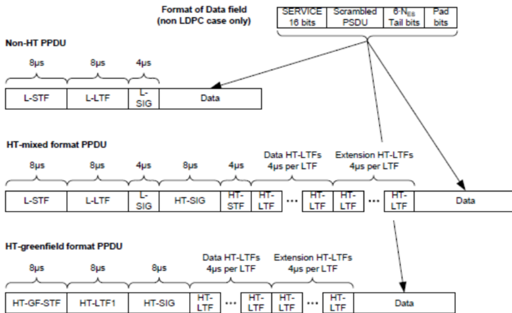
Figure 20-1—PPDU format
