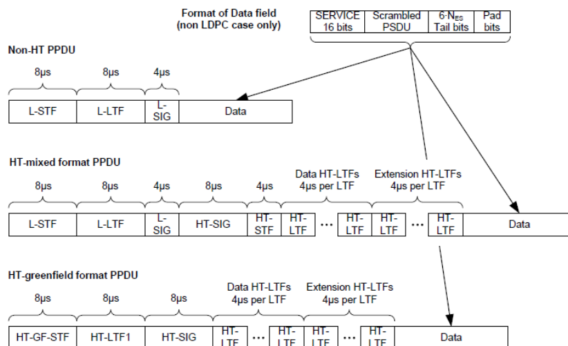
Figure 20-1—PPDU format
