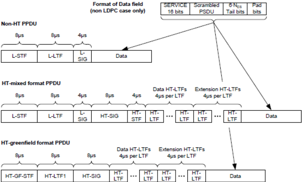
Figure 20-1—PPDU format
