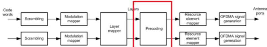
Figure 12: LTE downlink
