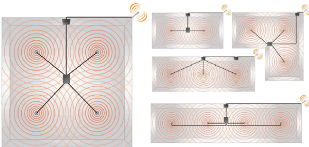
Sample weBoost Small Office PRO system multi-antenna setups
