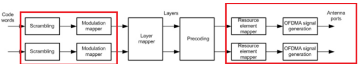
Figure 12: LTE downlink
