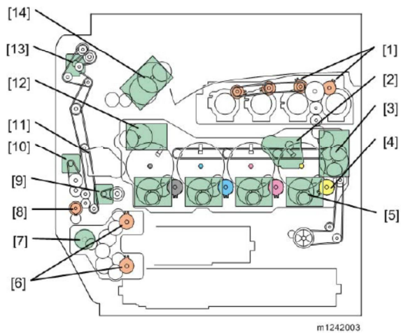
Drive Layout
