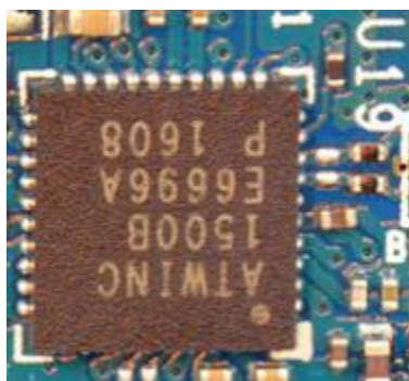
Amtel ATWINC1500B Wi-Fi module labeled 'U19' included within the Amazon Dash Button (the wireless transmitter). See https://mpetroff.net/2016/07/new-amazon-dash-button-teardown-jk29lp/#f1-2185
