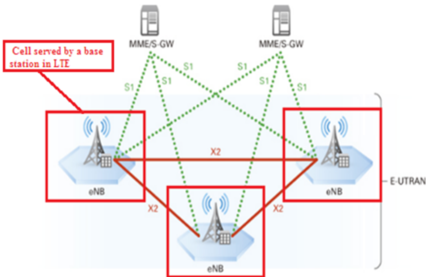
Figure 2 : E-UTRAN Architecture
