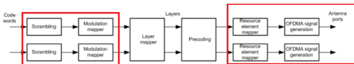
Figure 12: LTE downlink
