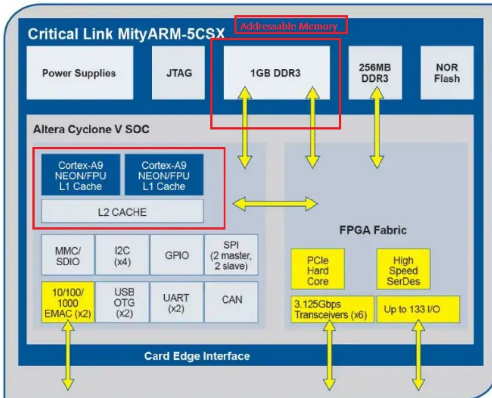
Block Diagram
