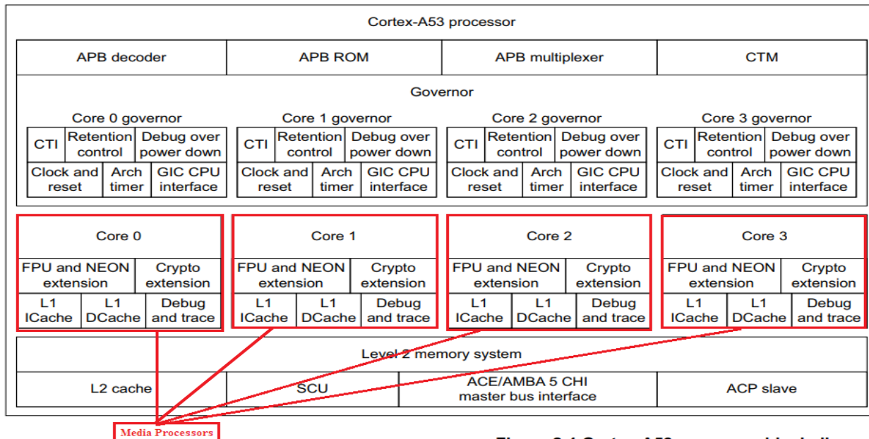
Figure 2-1 Cortex-A53 processor block diagram
