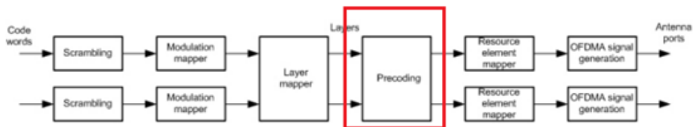
Figure 12: LTE downlink
