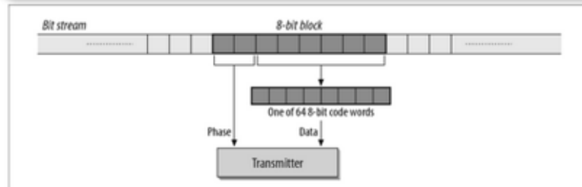
Figure 12-21. 802.11b transmission at 11 Mbps
