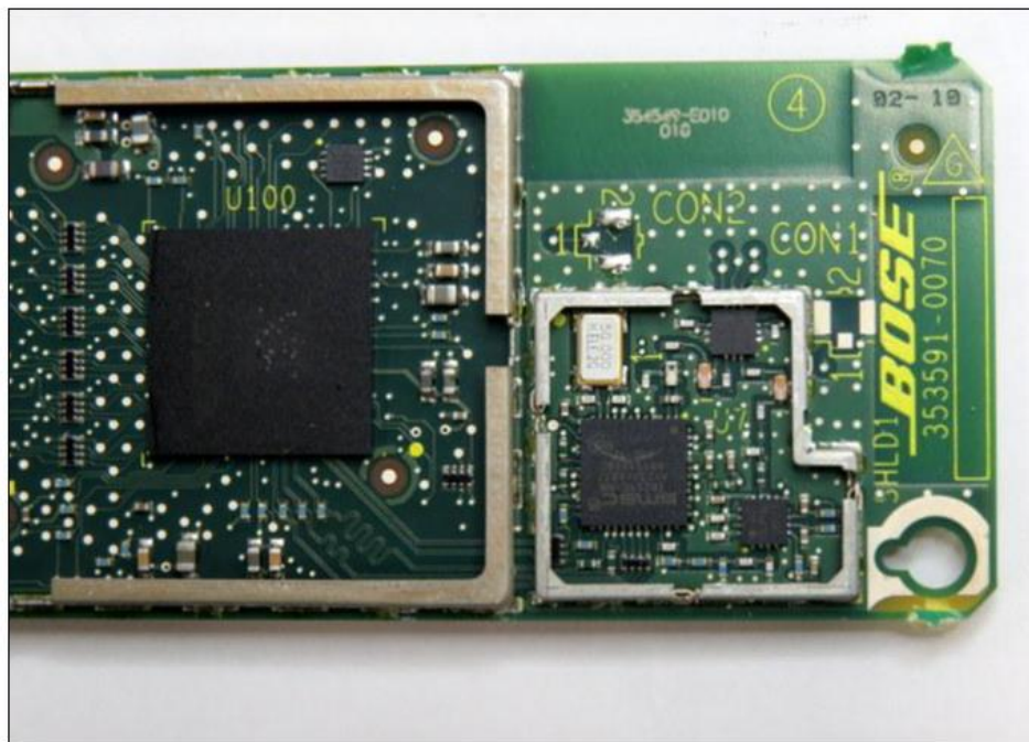
Bose Model 412568 Transceiver Module Internal Photos, BOSE TEARDOWN (the internal image above shows the Wi-Fi transceiver in the Bose Model 412568 component).
