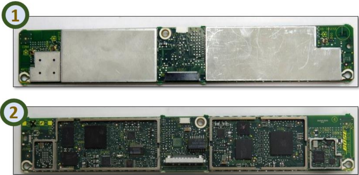
Bose Model 412568 Transceiver Module Internal Photos, BOSE TEARDOWN (Image “1” shows the Bose Transceiver Module with shielding; Image “2” shows the Bose Transceiver Module with the shielding removed) (annotation added).
