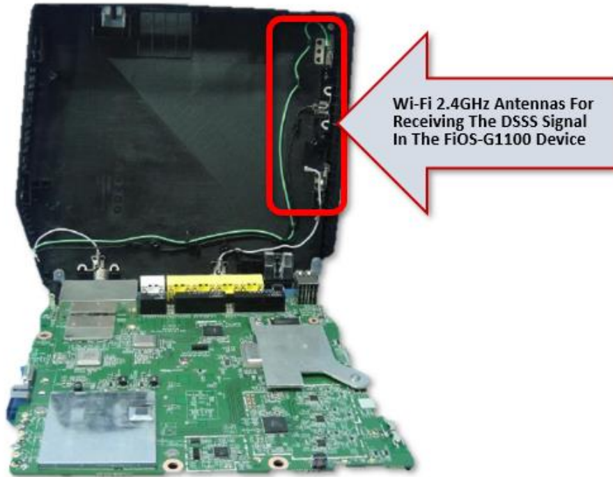
Verizon FiOS Quantum Gateway – FiOS-G1100 WiFi 2.4GHz Antennas, DEVICE TEARDOWN IMAGE (annotation added).
