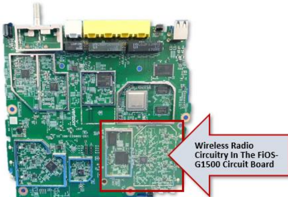
Verizon FiOS Quantum Gateway – FiOS-G1500 Circuit Board, DEVICE TEARDOWN IMAGE (annotation added).
