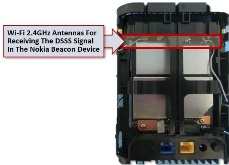
Nokia Beacon WLAN Antennas, DEVICE TEARDOWN IMAGE (annotation added).
