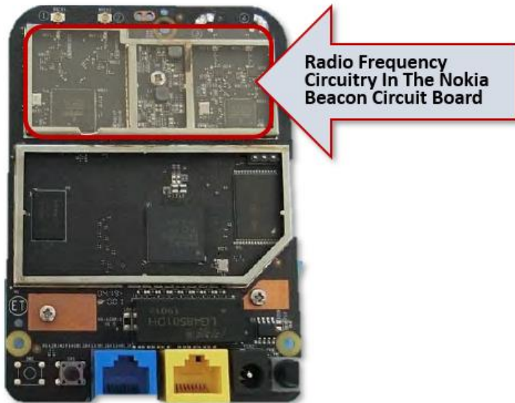
Nokia Beacon Circuit Board, DEVICE TEARDOWN IMAGE (annotation added).
