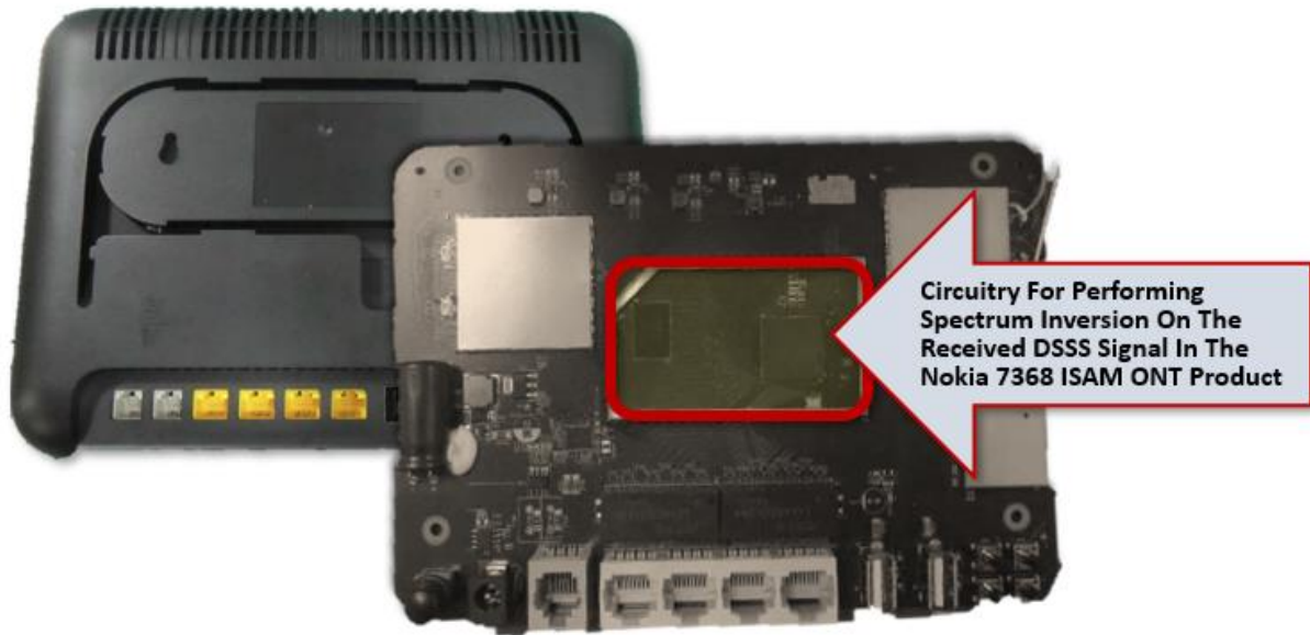
Nokia 7368 ISAM ONT G-240W-B, DEVICE TEARDOWN IMAGE (annotation added).
