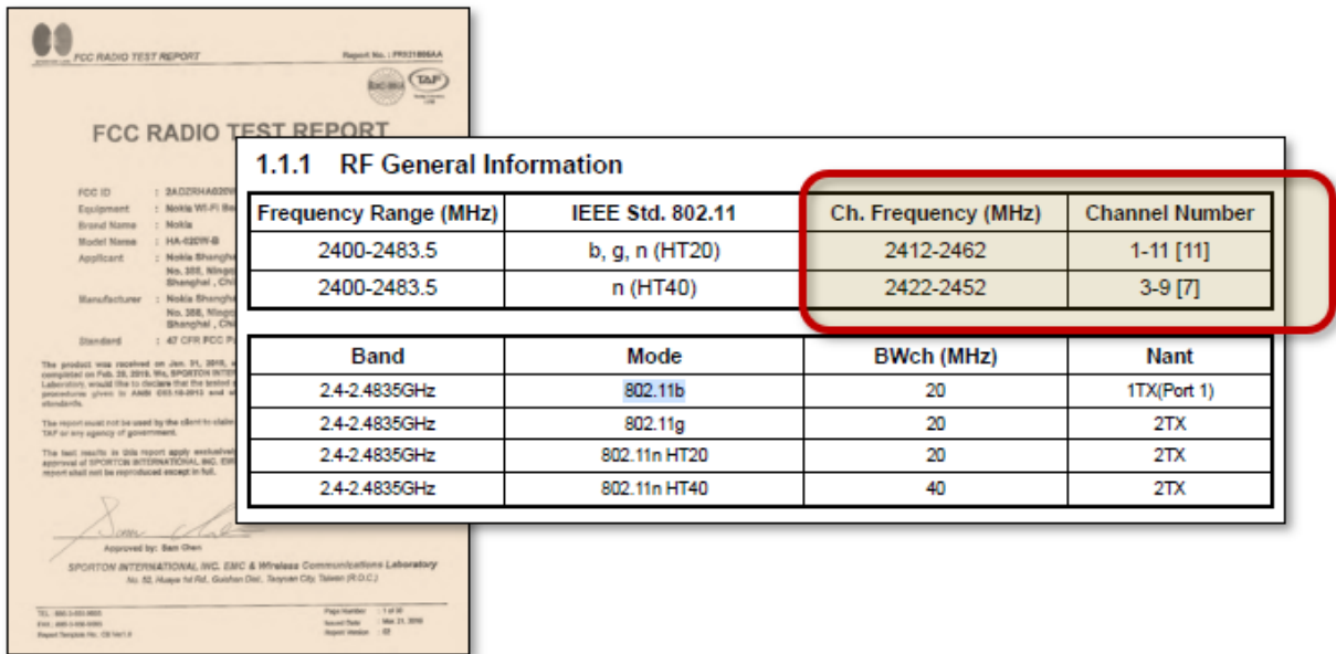
Nokia Wi-Fi Beacon, FCC ID 2ADZRHA020WB – 2.4GHz Test Report No. FR921805AA at 5 (March 21, 2019) (annotation added).
