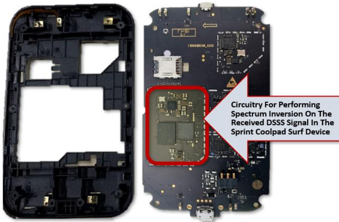
Sprint Coolpad Surf 2.4GHz Antennas , DEVICE TEARDOWN IMAGE (annotation added).
