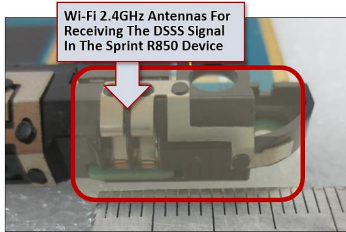
Sprint R850 Mobile Hotspot WLAN Antennas, DEVICE TEARDOWN IMAGE (annotation added).
