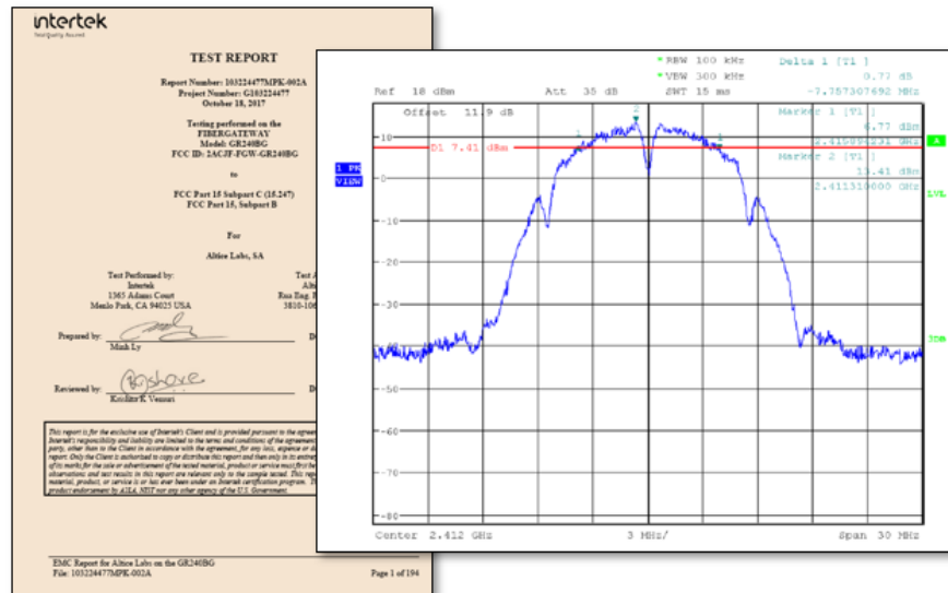
Altice FiberGateway FCC ID No. 2ACJF-FGW-GR240BG, FCC TEST REPORT RE WiFi 2.4 GHz NO. 103224477MPK-002A at 12 (October 18, 2017) (showing channel 1 of the 802.11b frequency at 2412MHz).
