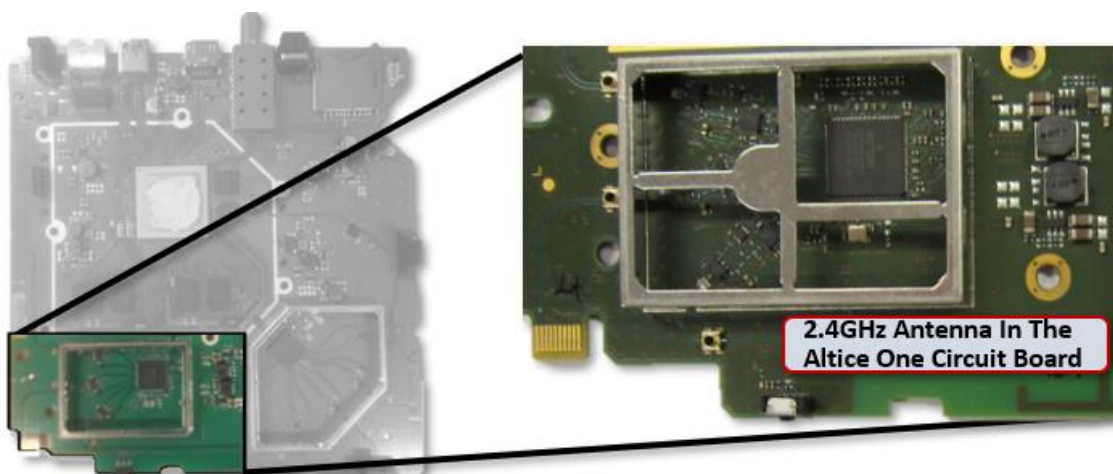
Altice One Mini 2.4GHz Antenna Location, DEVICE TEARDOWN IMAGE (annotation added).
