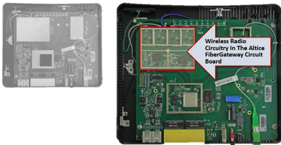
Altice FiberGateway Model No. GR240BG Circuit Board, DEVICE TEARDOWN IMAGE (annotation added).
