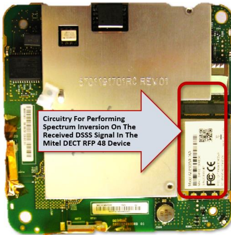
Mitel SIP-DECT Base Station RFP 48 Circuit Board, DEVICE TEARDOWN IMAGE (annotation added).
