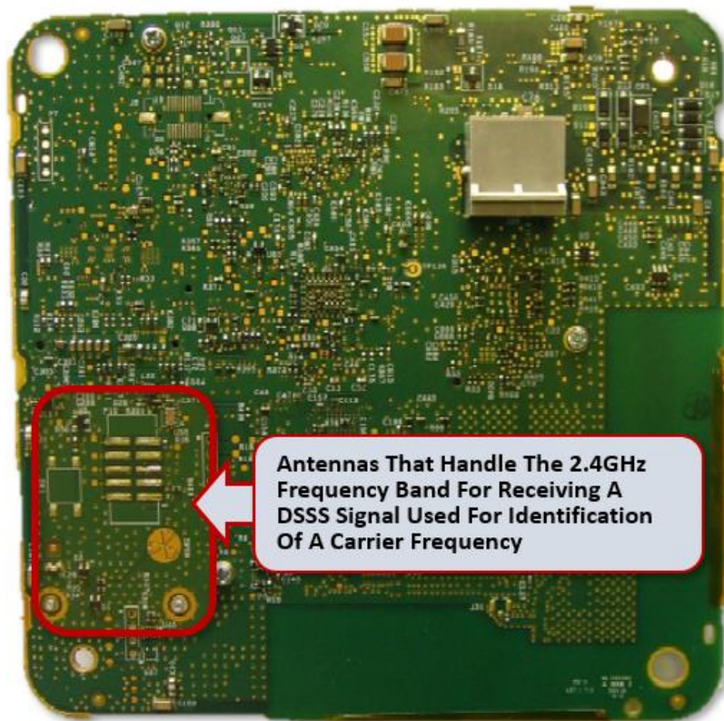
Mitel SIP-DECT Base Station RFP 48, DEVICE TEARDOWN IMAGE (annotation added) (showing the antennas in the device).
