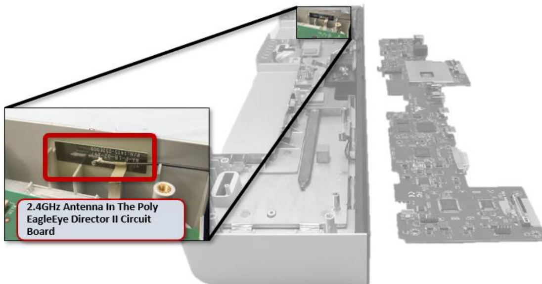
Poly EagleEye Director II 2.4GHz Antenna Location, DEVICE TEARDOWN IMAGE (annotation added).
