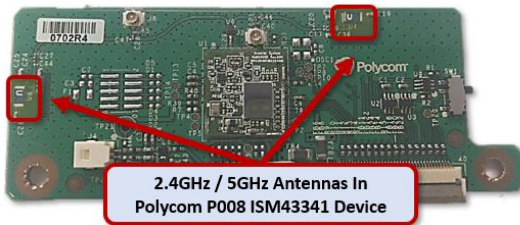
Polycom P008 Embedded ISM SIP Application Module WiFi Antennas, Device TEARDOWN IMAGE (annotation added).
