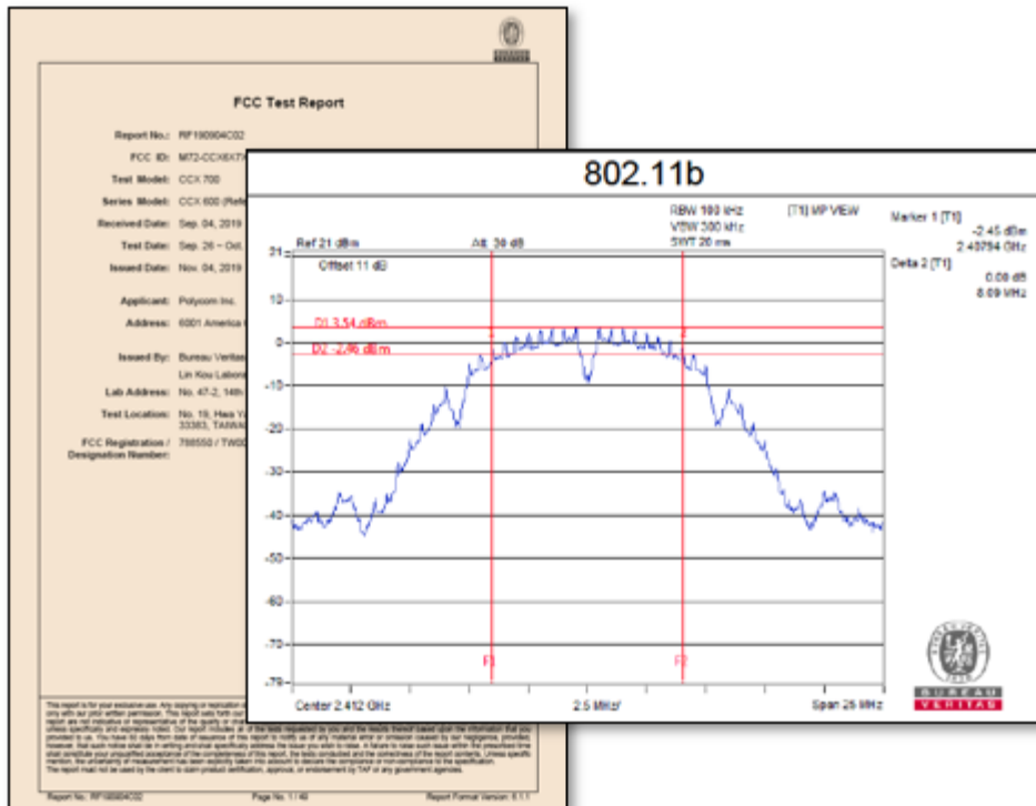
Poly CCX 600 FCC ID No. M72-CCX6X7X, FCC TEST REPORT RE WiFi No. RF190904C02 (November 4, 2019) (showing channel 1 of the 802.11b frequency at 2412MHz).
