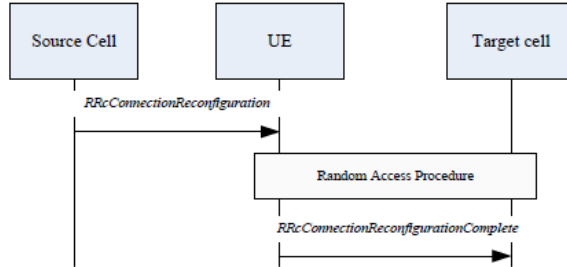
Figure 4-4 Intra-eNodeB Handover
