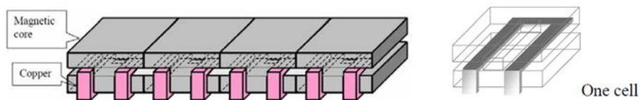
Figure 4.15 A scalable multi-phase surface mount coupling inductor structure proposed by Volterra in [77]
