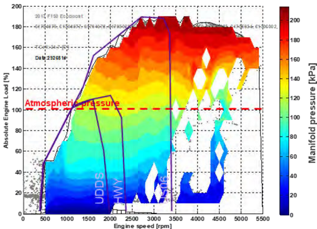
Figure 31: Manifold pressure and boost map as a function of the engine speed and load
