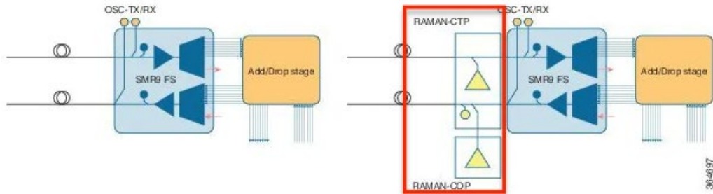
Figure 12. Terminal Node Configuration with SMR9 FS Card
