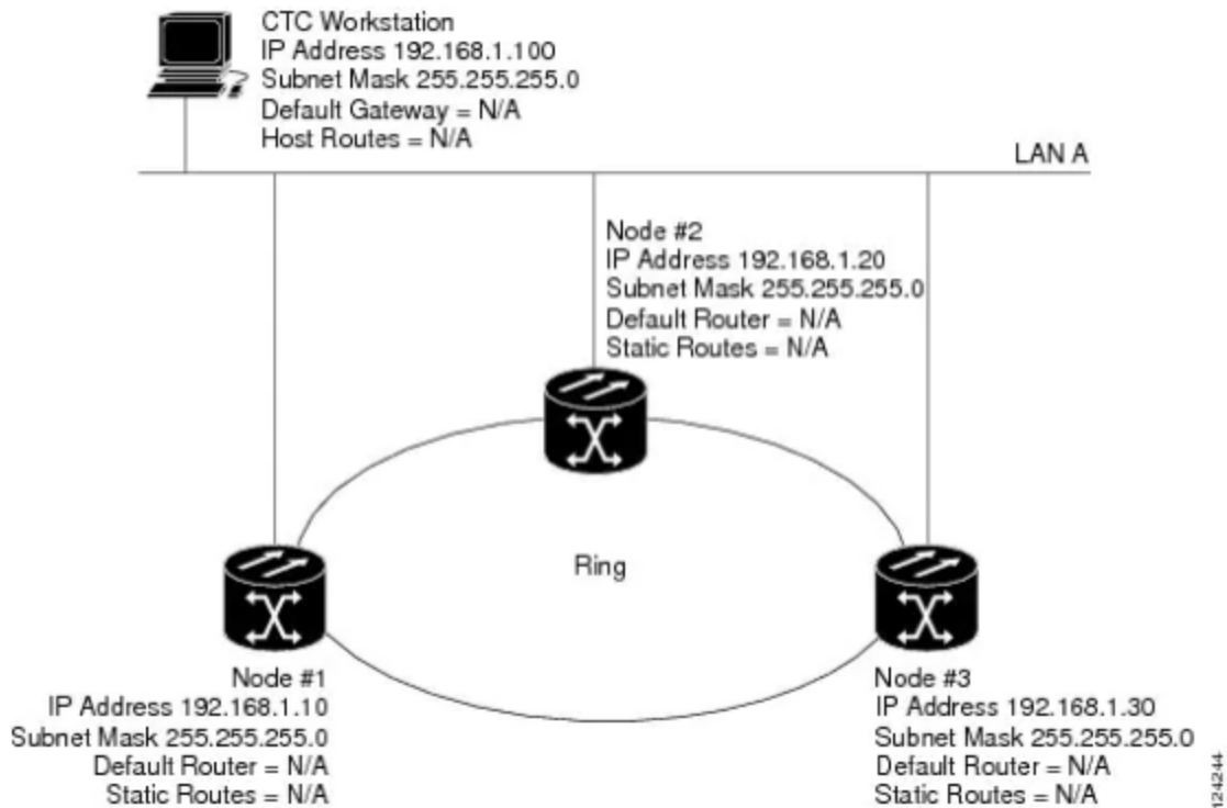
Figure 1. Scenario 1: CTC and NCS on Same Subnet (ANSI and ETSI)
