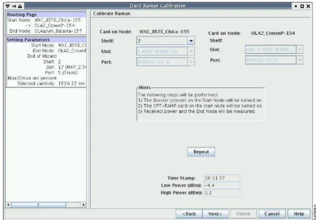
Figure 10. Calibrating Raman Amplification
