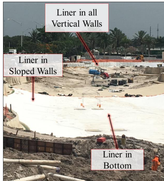
Figure 18: Liner covering vertical walls, sloped walls, and bottom
