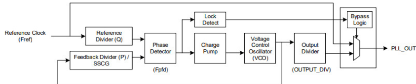
Figure 18-3. PLL with SSCG and Fractional Operation
