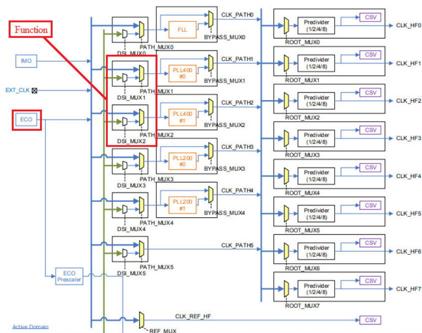
Figure 2. Block Diagram
