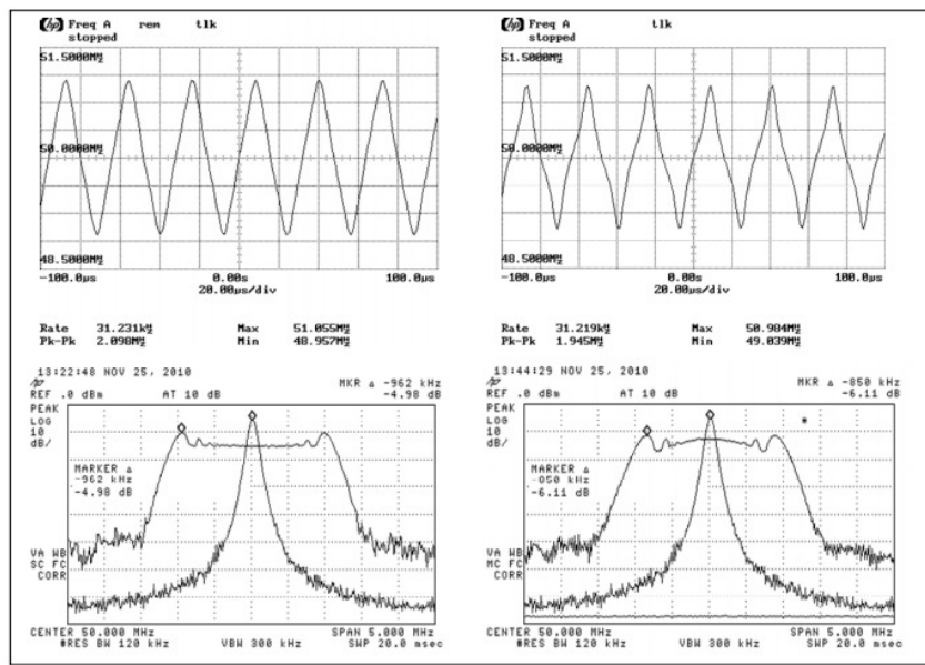
a) Linear Spread profile & Output Spectrum
