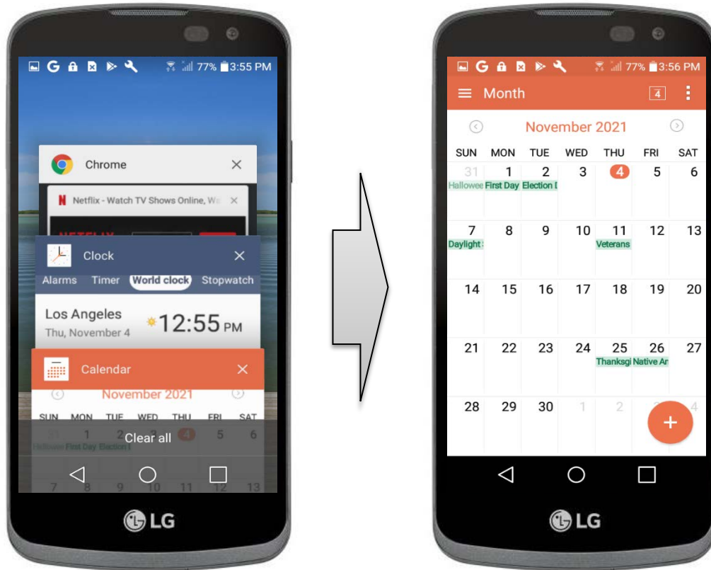
Fig. 26. Illustrations of a three-dimensional space displaying images of three open applications (left) and a two-dimensional space displaying the Calendar application in response to user input (right).
