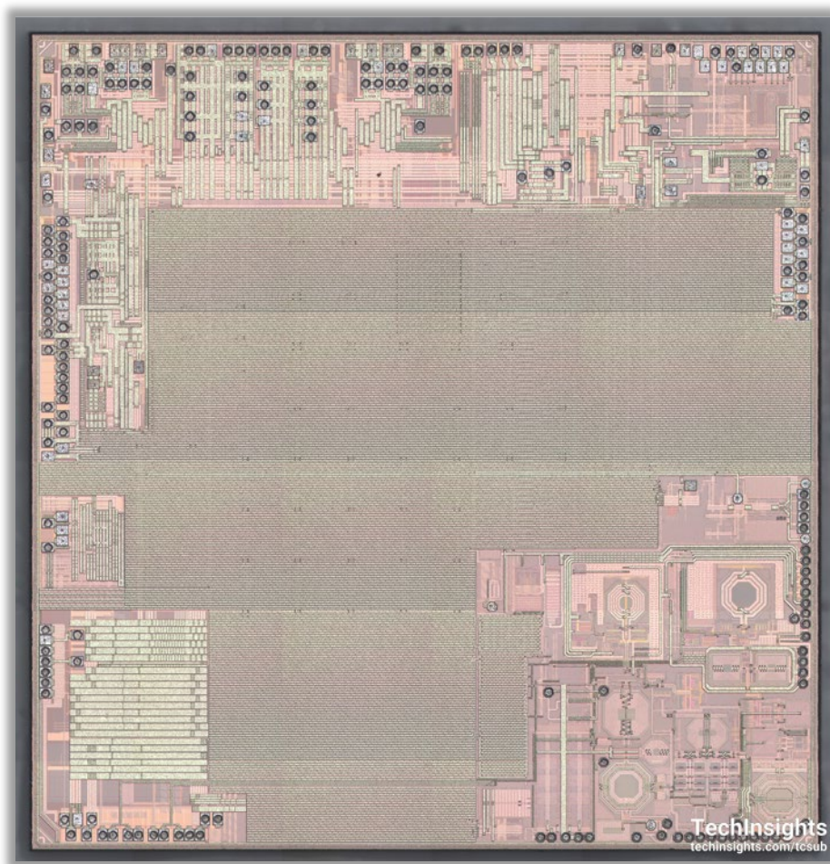
Realtek RTL8763B Processor Die with Integrated Circuits.
