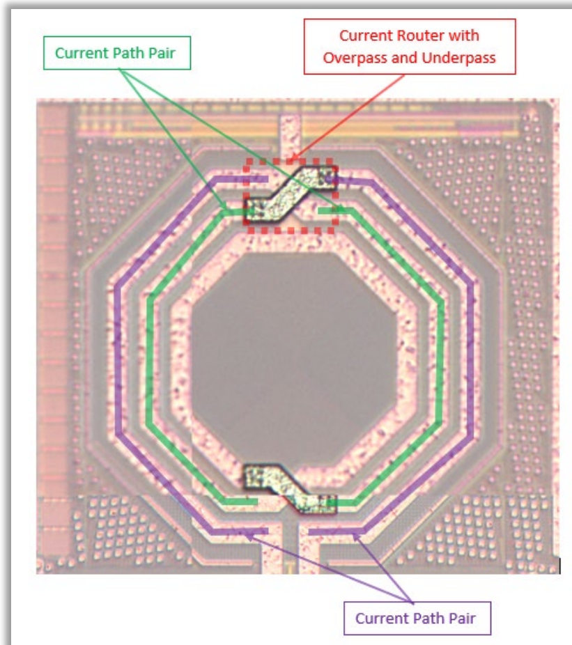
Realtek RTL8763B Processor Inductor
