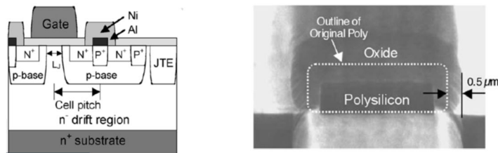
Fig. 6. SEM image of the oxidized polysilicon finger used as a self-aligned mask for the source implant.
