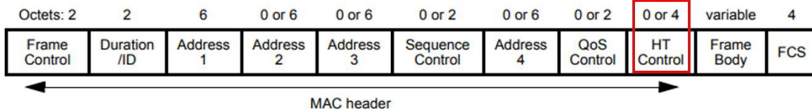
Figure 9-1—MAC frame format
