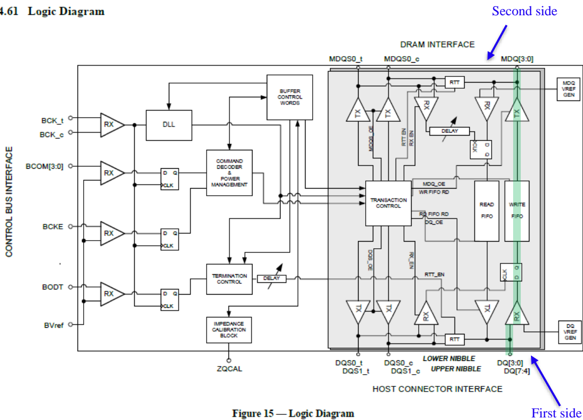
Figure 15 — Logic Diagram
