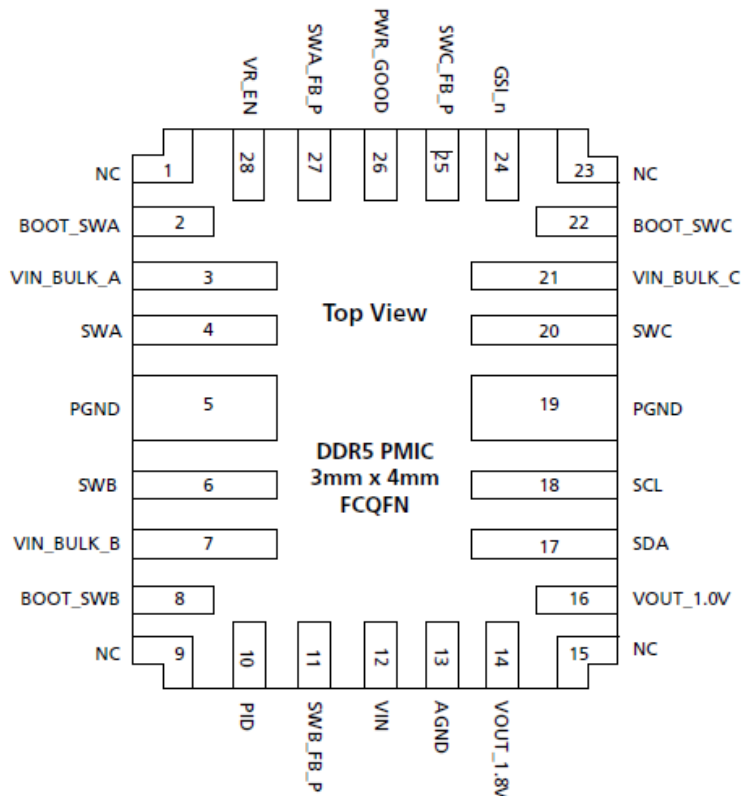
Figure 1: PMIC Package
