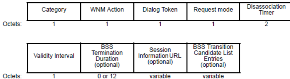
Figure 9-701—BSS Transition Management Request Action field format
