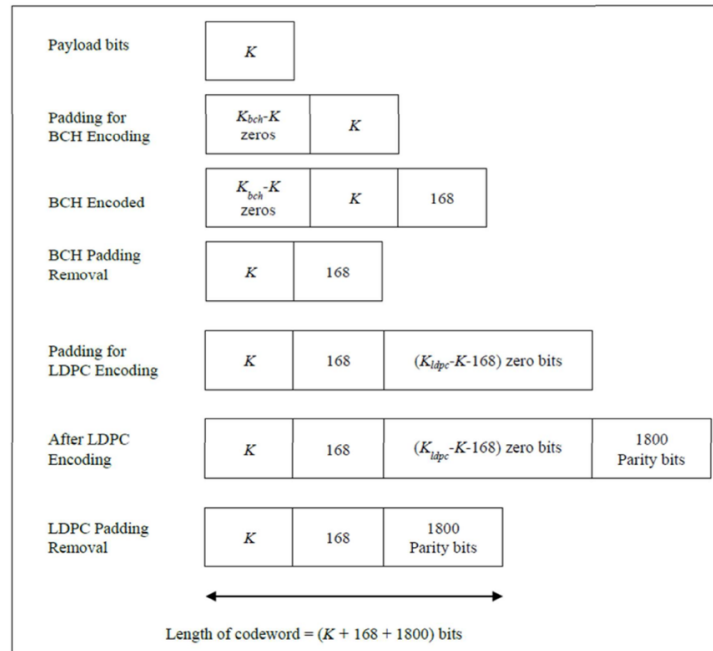
Figure 47 - Padding Process
