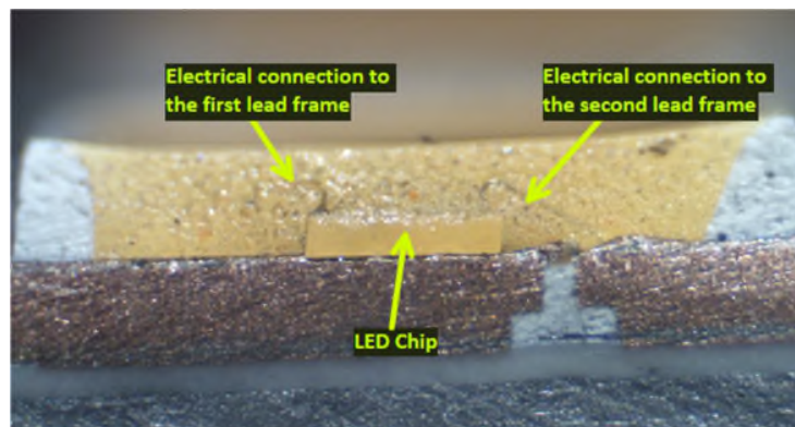
Figure 1B - 6 Wedge – Z9302-OBO-LED
