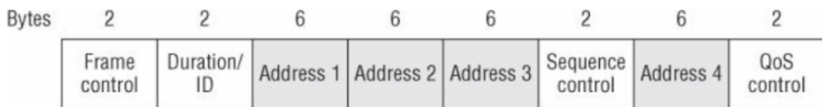
Figure 9.3 802.11 MAC header
